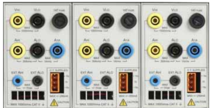
PA4000 Rear Panel - Input Modules
